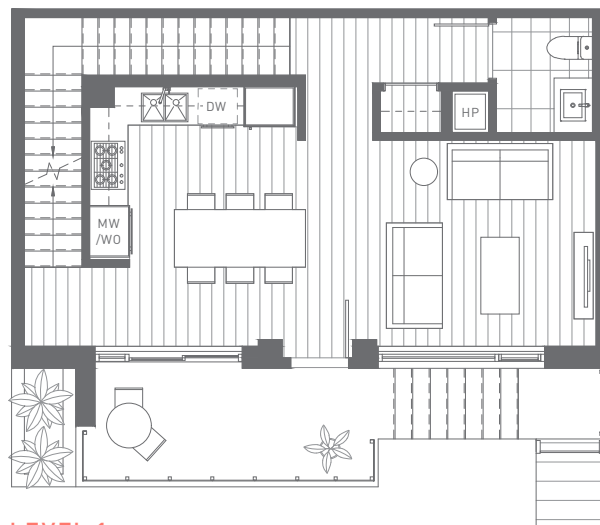
LEVEL 1
