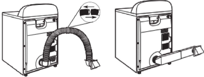
Over-The-Top installation (also available with one offset elbow)
